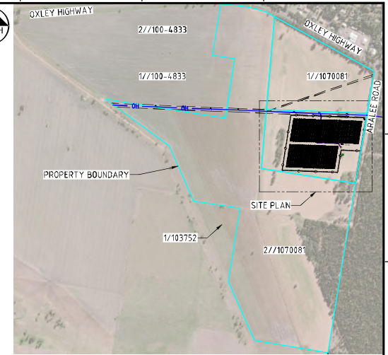
KEY PLAN SCALE 1:10000
