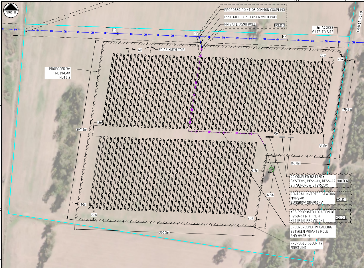
SITE PLAN SCALE 1:1250
